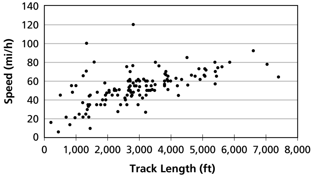
Track Length and Speed of 150 Wood and Steel Coasters
